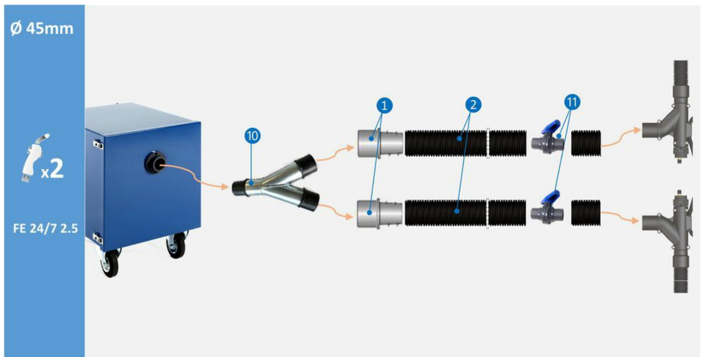
Accessories configuration for two users, 45mm welding machine connection. (10) Branch 50/50/50, art.no. 55999420 (1) Hose Coupler M50-44P, art.no. 55999418 (2) Hose Superflex Ø45mm Black 5m, art.no. 55999411 (11) Ball valve 44mm, art.no. 55999422
